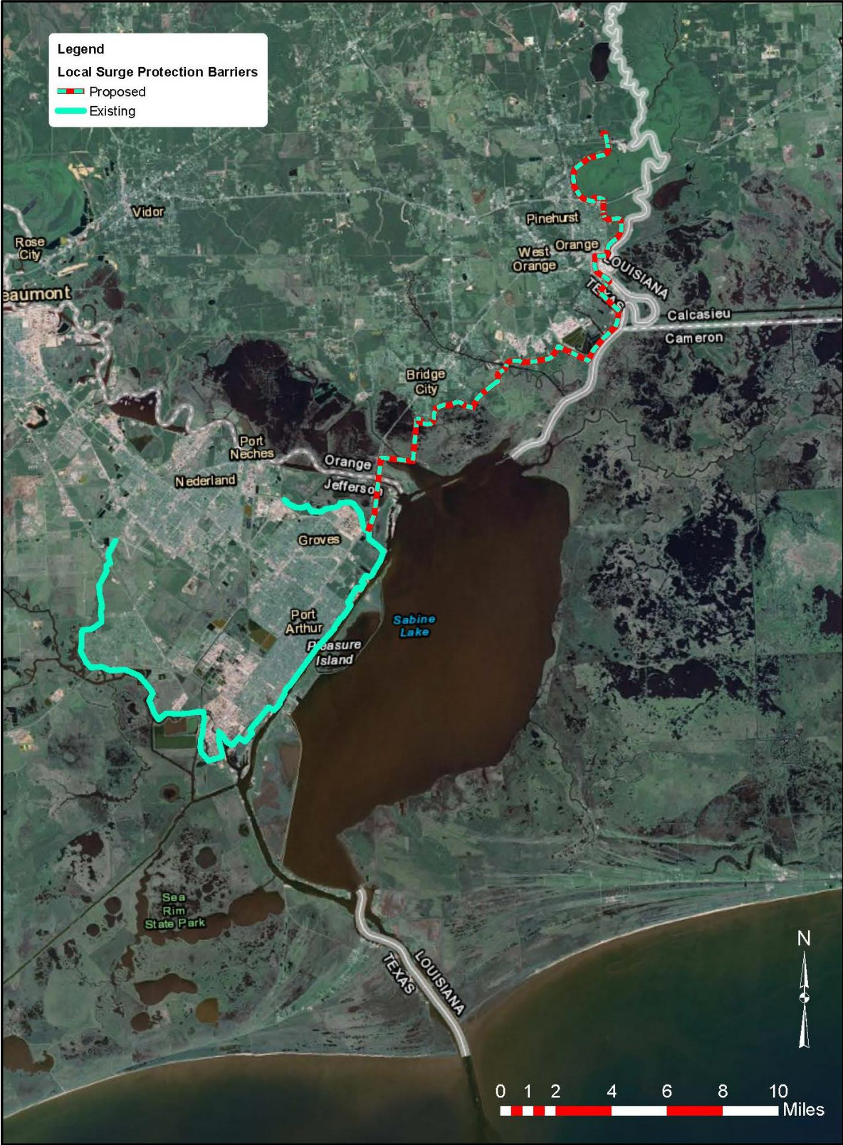
Figure 6-1. Gate Alternative
