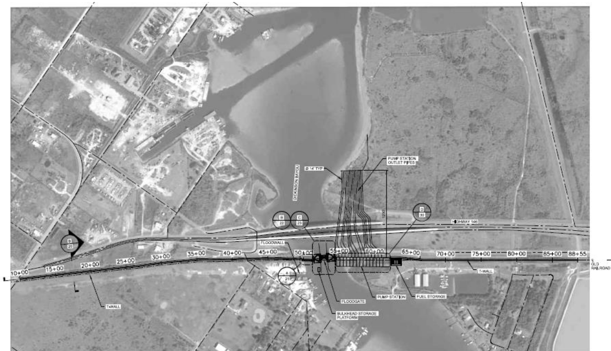
Figure 2-55: Dickinson Bay Gate Closure System with Pump Station Footprint (Annex 7)
