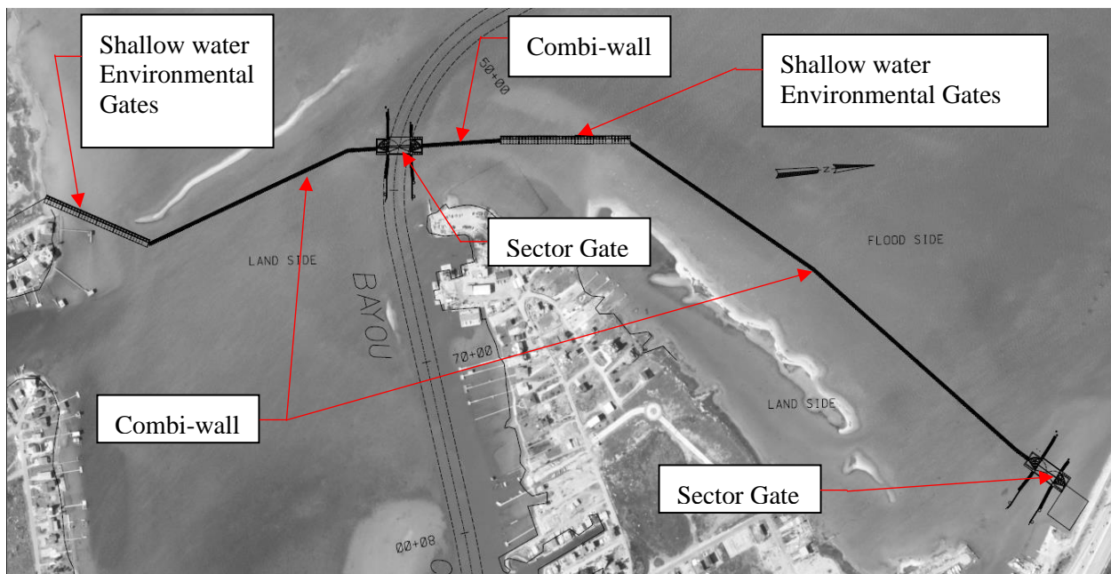
Figure 6-16: Offatts Bayou Crossing
