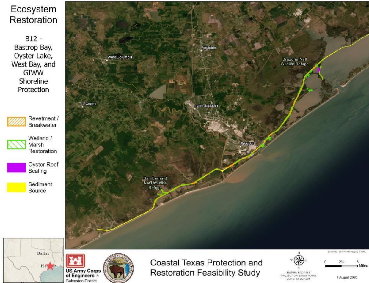
Figure 7-4: B-12 – West Bay and Brazoria GIWW Shoreline Protection
