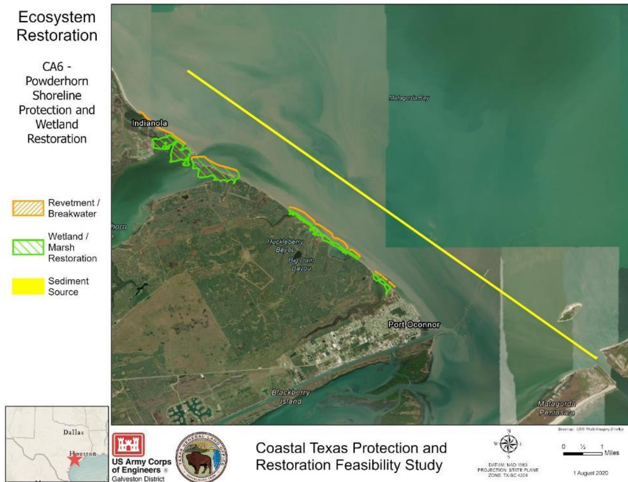
Figure 7-6: CA-6 – Powderhorn Shoreline Protection and Wetland Restoration
