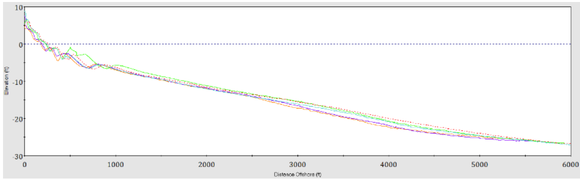
Figure 5-2: Five morphologically similar 2016 reaches identified on Galveston, profiles are averaged in BMAP to create representative cross section
