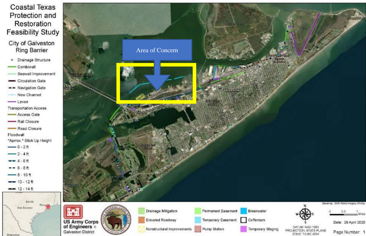
Figure 4-14: Offshore Breakwater
