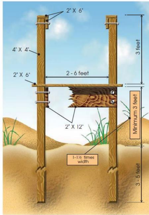
Figure 4-4: Typical Walkover Section
