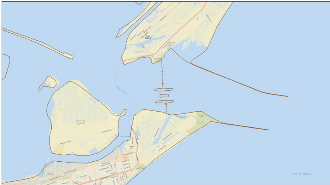
Figure 2-56: Revised Storm Surge Barrier Modeled (2019PWP) for the AdH model domain.
