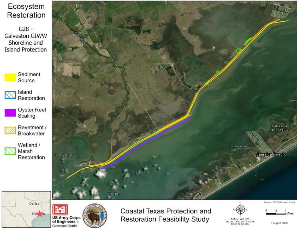
Figure 7-2: G-28 – Bolivar and West Bay GIWW Shoreline and Island Protection West
