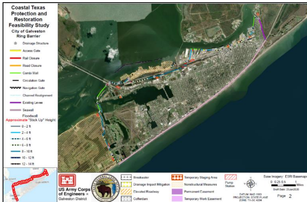
Figure 3-6: City of Galveston Ring Barrier (Outside of Seawall Portion, (Annex 17 has Details)
