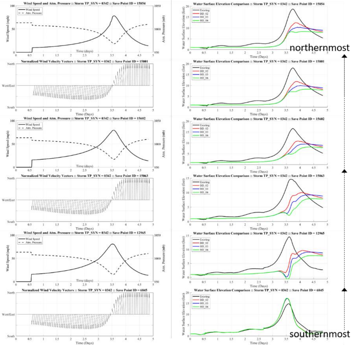
Figure 2-31: Comparison of water surface elevation for storm 342 (right hand side) at six (6) save point locations for four (4) different configurations. The left-hand side shows the corresponding wind direction (as normalized vectors), wind speed and atmospheric pressure
