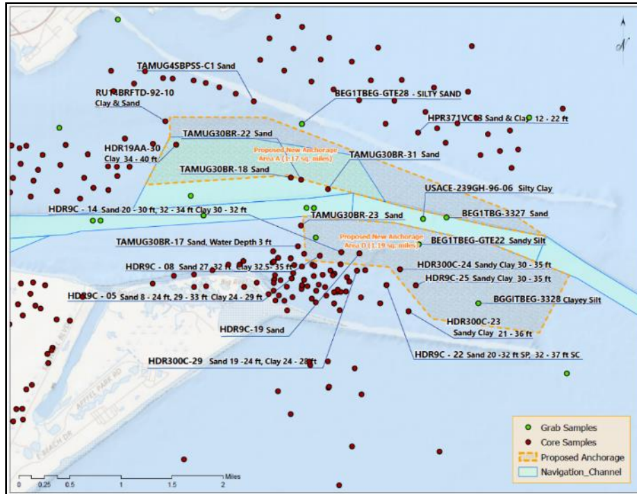
Figure 3-14: Proposed Galveston Harbor Entrance Channel and Anchorage Area Improvements (Source: https://gisweb.glo.texas.gov/txsed/index.html )
