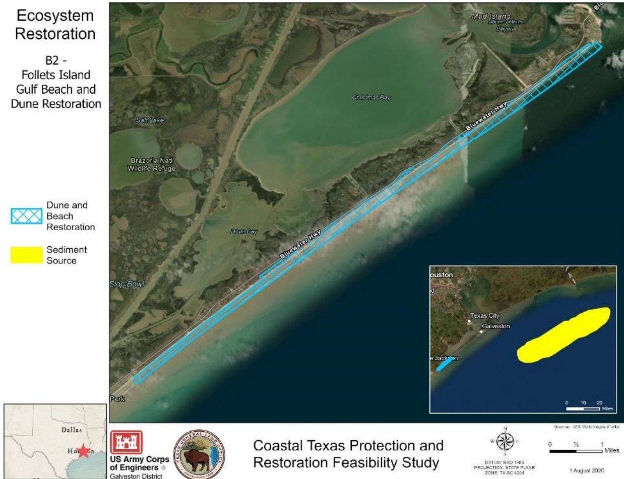
Figure 7-3: B-2 – Follets Island Gulf Beach and Dune Restoration
