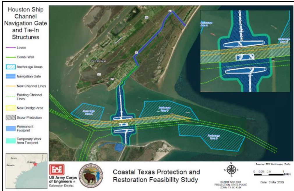
Figure 3-1: Bolivar Road Surge Barrier System
