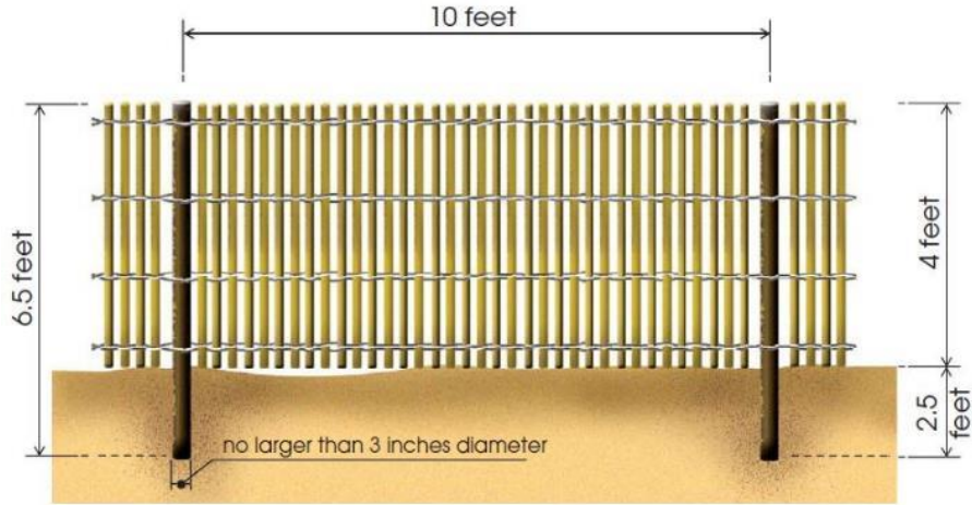
Figure 4-3: Typical Sand Fencing Installation Detail
