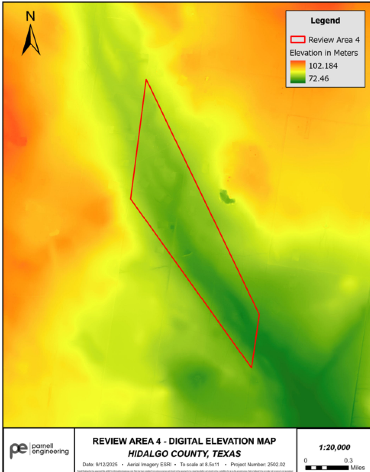
Figure 6: Digital Elevation Model
