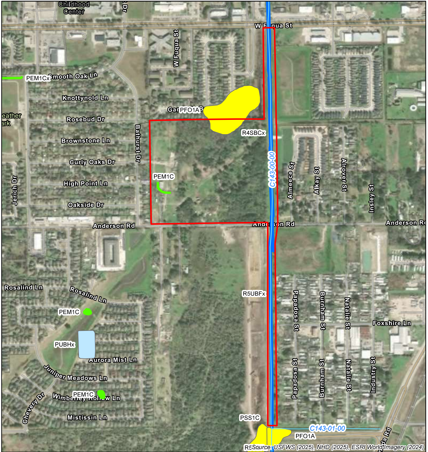
FIGURE 5 NATIONAL WETLAND INVENTORY MAP TRIBUTARY C143-00-00 CONVEYANCE IMPROVEMENTS PROJECT ID C140-00-00-E001 HOUSTON, HARRIS COUNTY, TEXAS 77053
