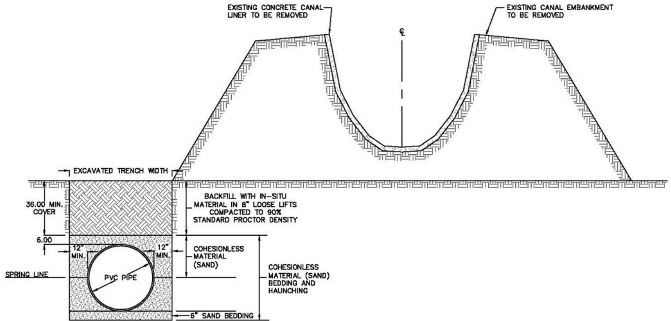
Pipeline Installation Typical Section.
