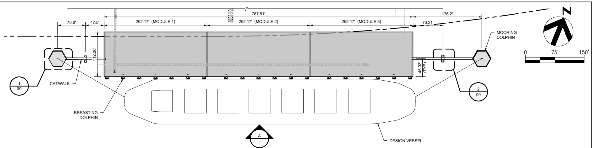
ENLARGED PLAN - BULK CARRIER DOCK 1" = 150'
