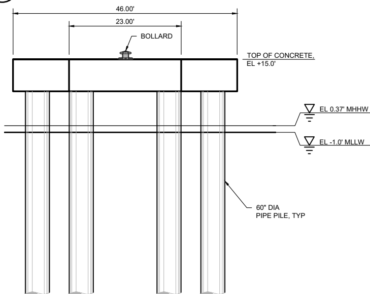
A - ELEVATION 1" = 20'
