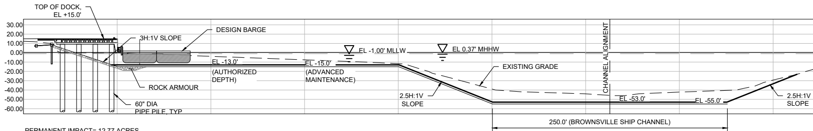
CROSS SECTION - BARGE DOCK BASIN B 05 1" = 100'
