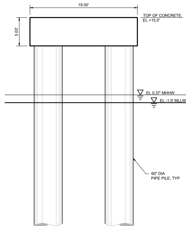
B - ELEVATION 1" = 10'
