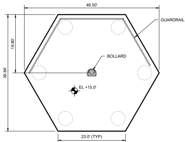
1 07 ENLARGED PLAN - MOORING DOLPHIN 1" = 20'
