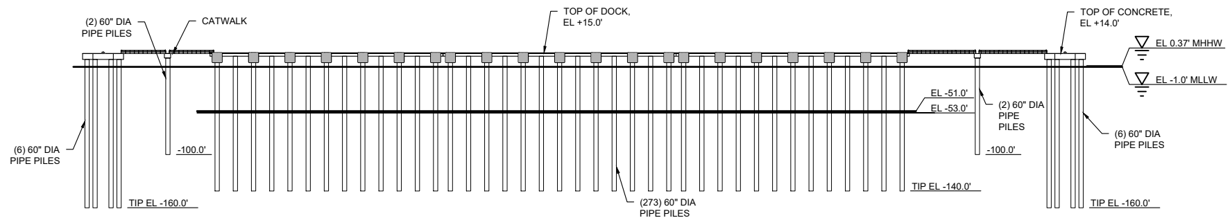
ELEVATION - BULK CARRIER DOCK 1" = 150'
