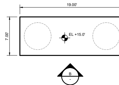
2 07 ENLARGED PLAN - CATWALK SUPPORTING PIER 1" = 10'
