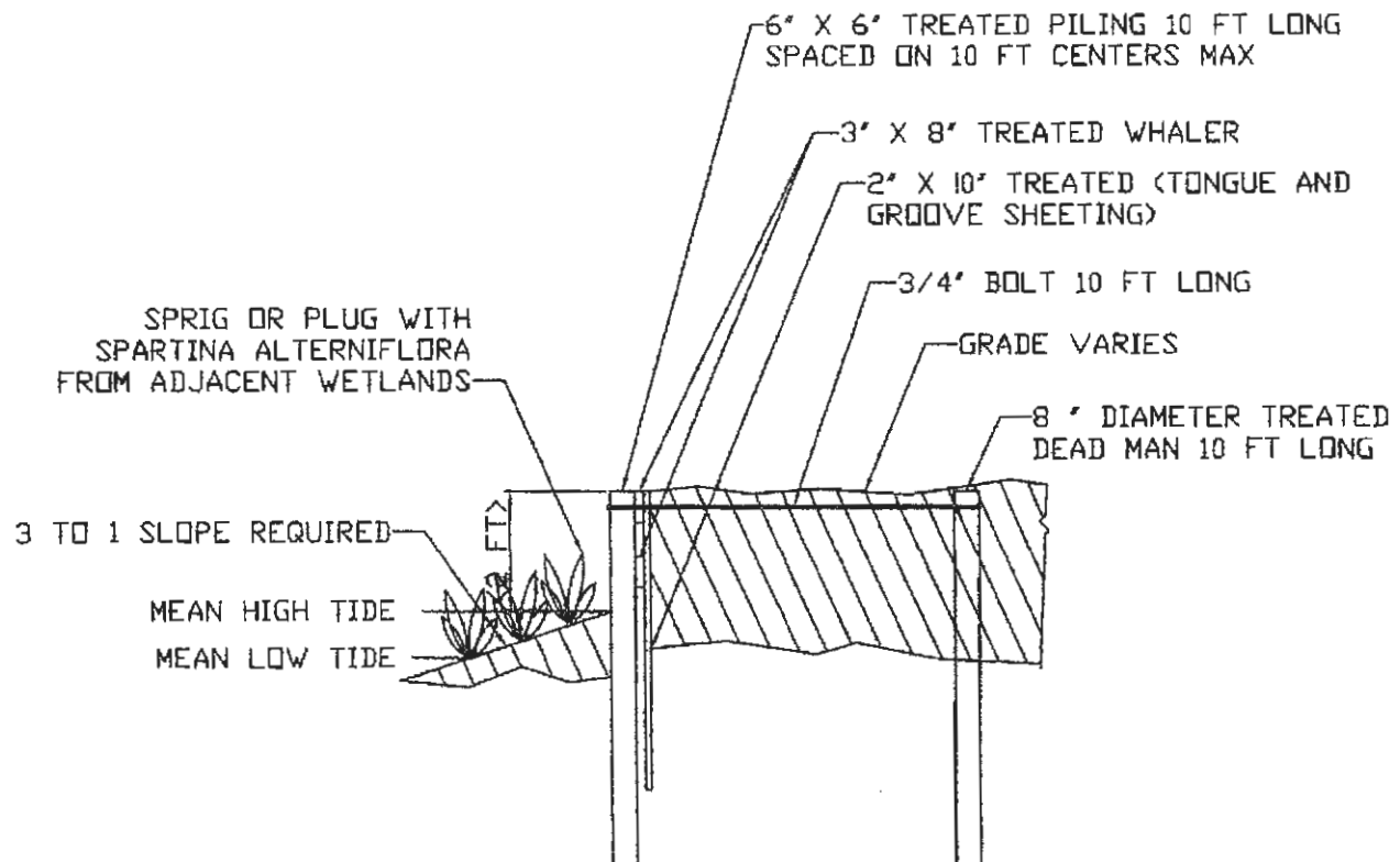
BULKHEAD CROSS SECTION
