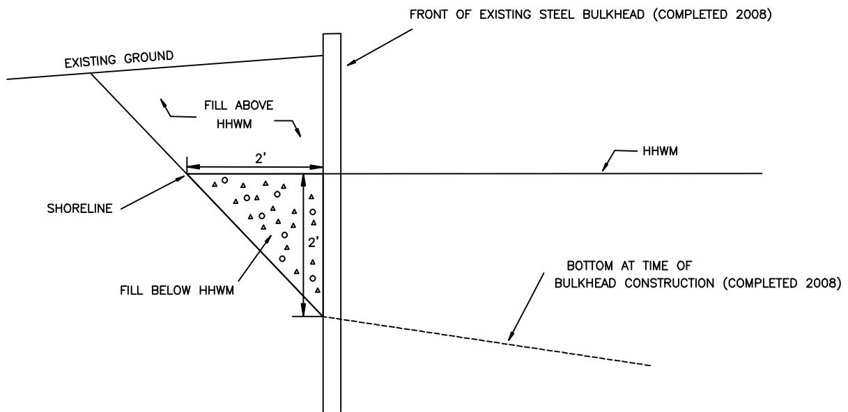
CROSS SECTION GG TYPICAL FILL BEHIND BULKHEAD
