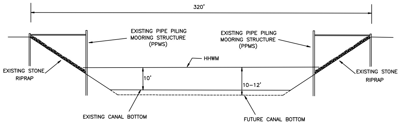
CROSS SECTION CC
