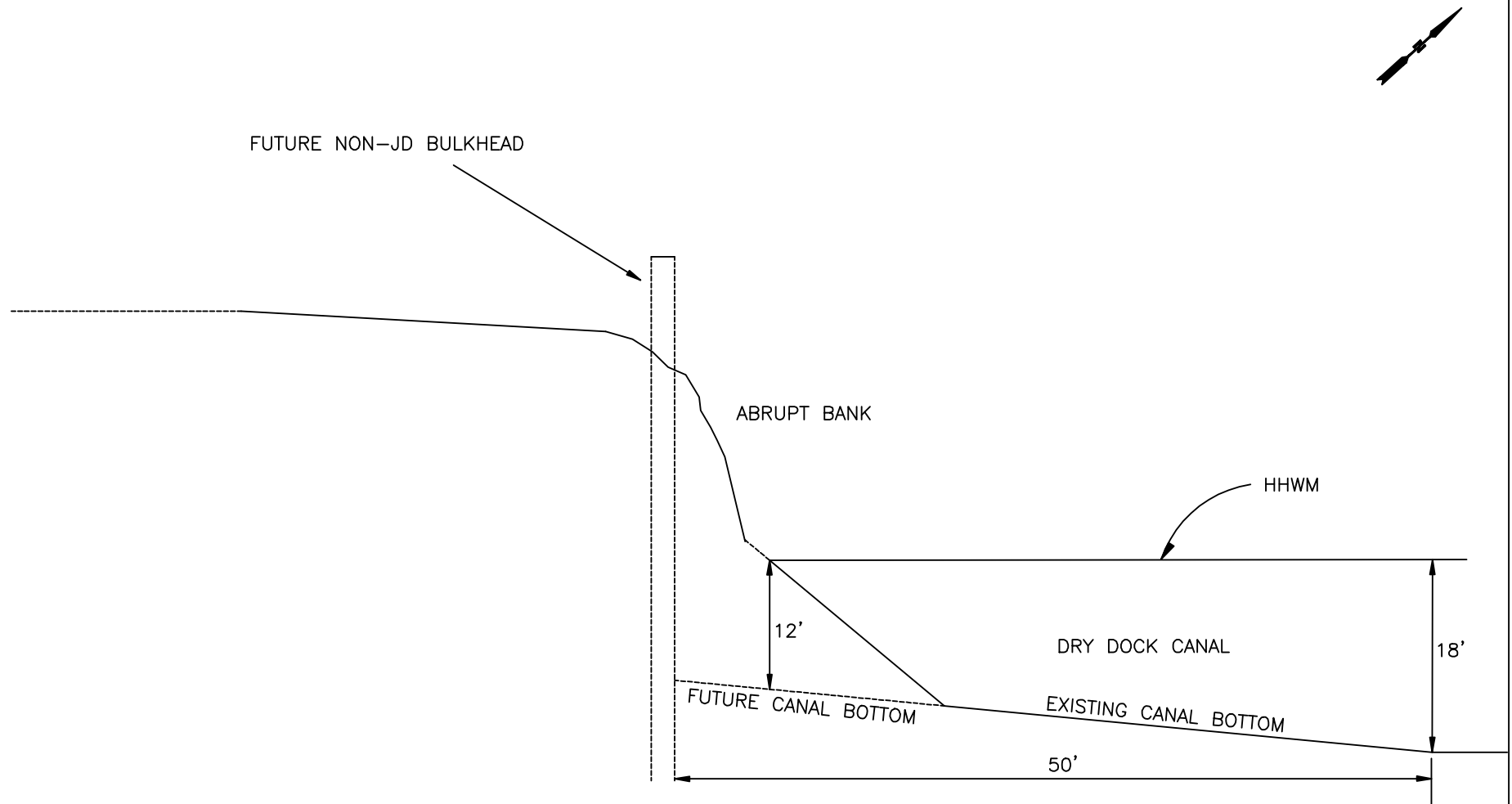
SWG-2001-01994 TEXAS BARGE AND BOAT CROSS SECTION FF AT AOC "D"
