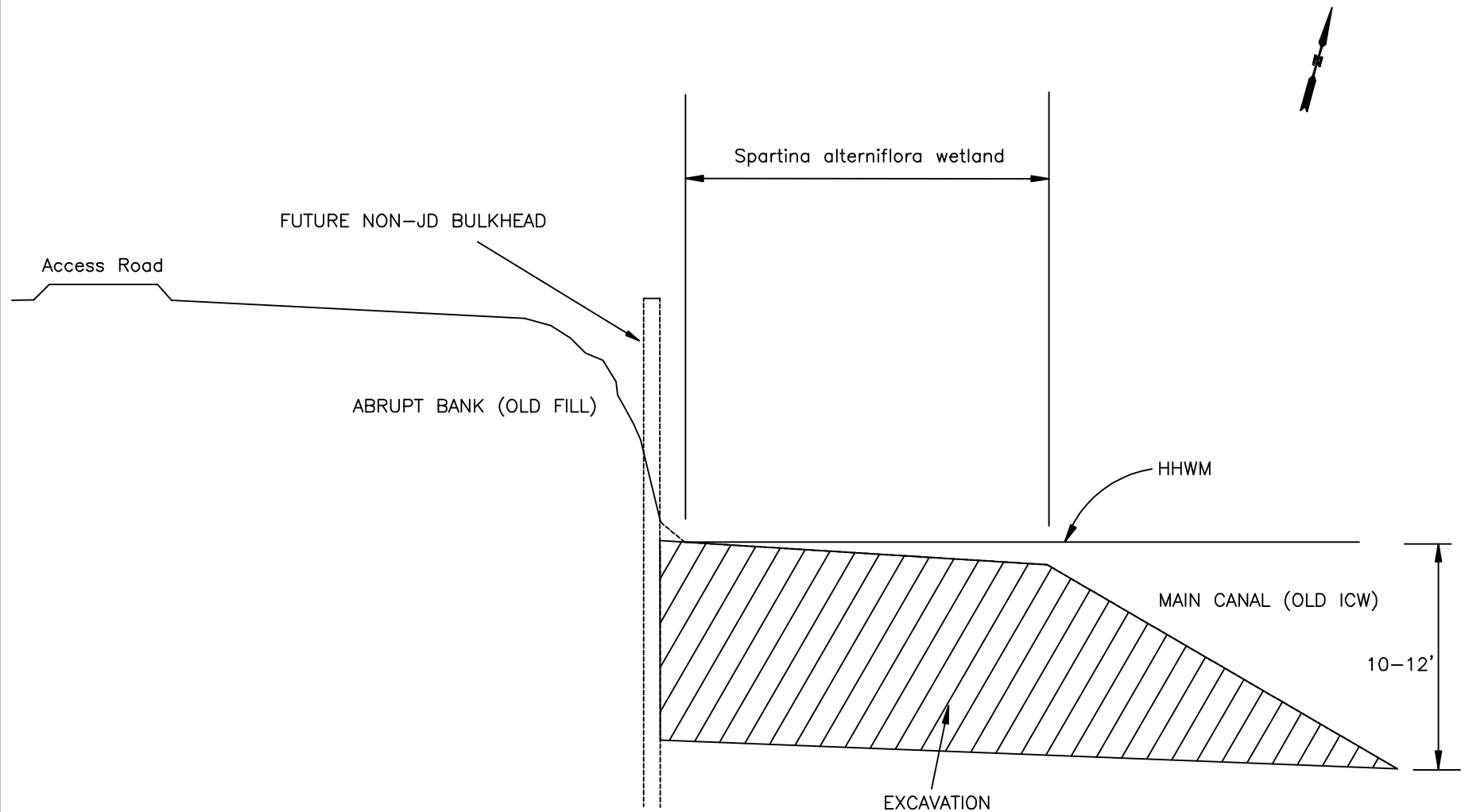
SWG-2001-01994 TEXAS BARGE AND BOAT CROSS SECTION AA AT AOC "B"
