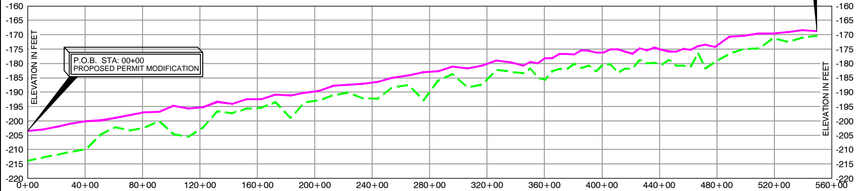
SEG 20125 - PROFILE VIEW HORIZONTAL SCALE: 1" = 6,000' VERTICAL SCALE: 1" = 40'
