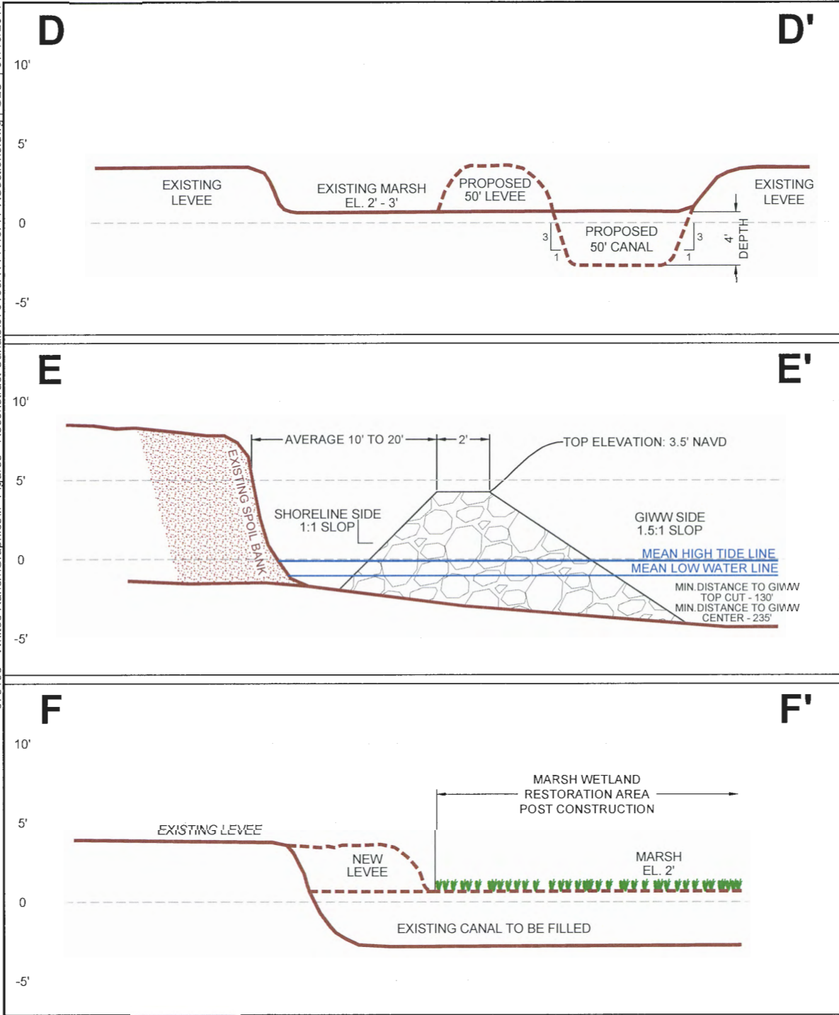
FIGURE 22 CROSS SECTIONS D-D' & E-E' OUTFALL AND POST CONSTRUCTION CROSS SECTION F-F' OUTFALL CANAL 2 - WHITE RANCH RECONSTRUCTION OF OUTFALL CANALS CHAMBERS AND JEFFERSON COUNTIES, TEXAS
