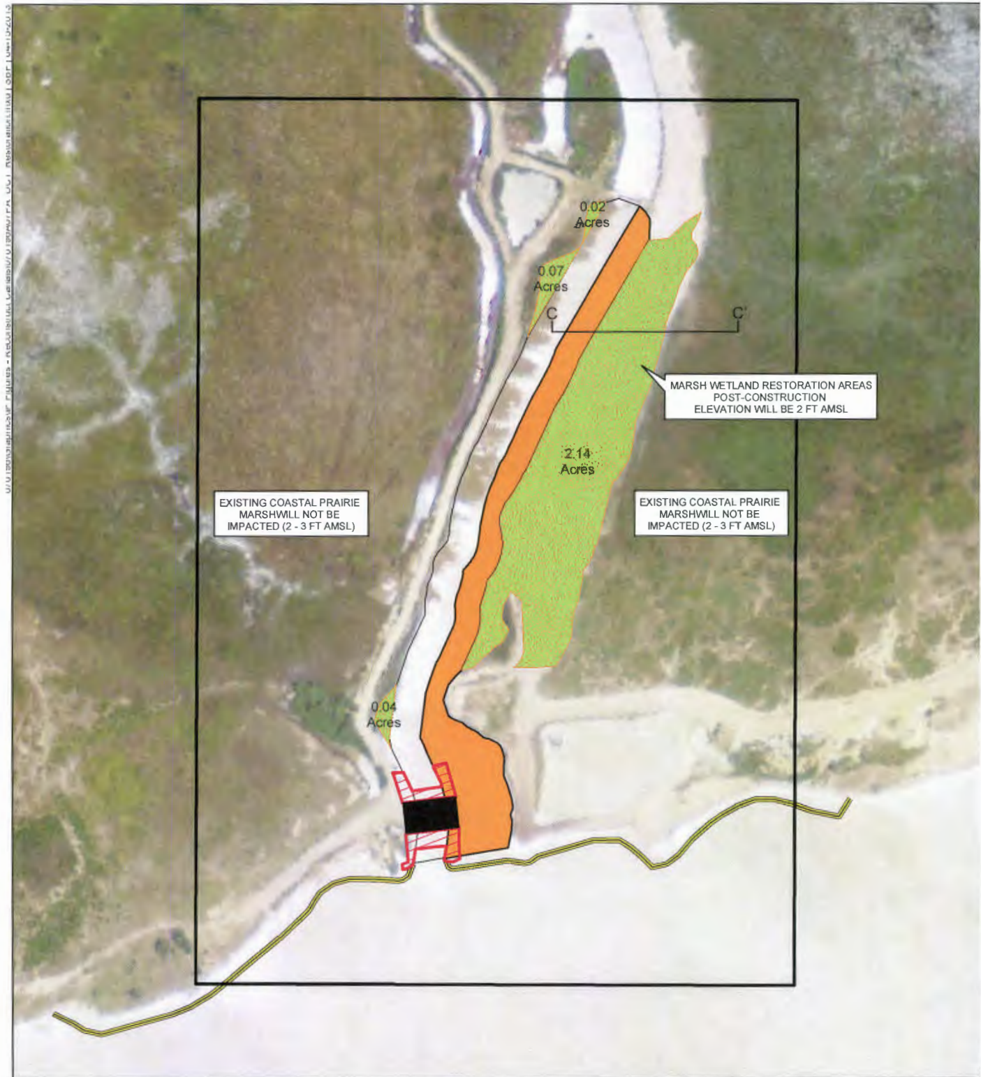
FIGURE 7 REV OUTFALL CANAL 1 RESTORATION PLAN CHAMBERS AND JEFFERSON COUNTIES, TEXAS SWG-2008-00352
