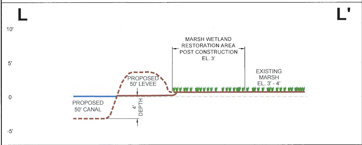
FIGURE 26 REV CROSS SECTIONS J-J' & K-K' OUTFALL AND POST CONSTRUCTION CROSS SECTION L-L' OUTFALL CANAL 4 - WHITE RANCH RECONSTRUCTION OF OUTFALL CANALS CHAMBERS AND JEFFERSON COUNTIES, TEXAS
