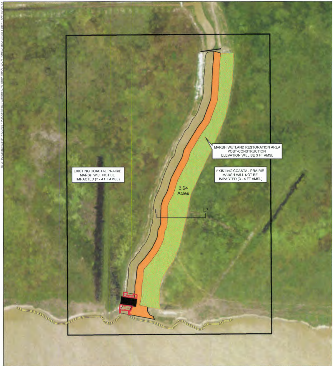
FIGURE 19 REV OUTFALL CANAL 4 RESTORATION PLAN CHAMBERS AND JEFFERSON COUNTIES, TEXAS SWG-2008-00352
