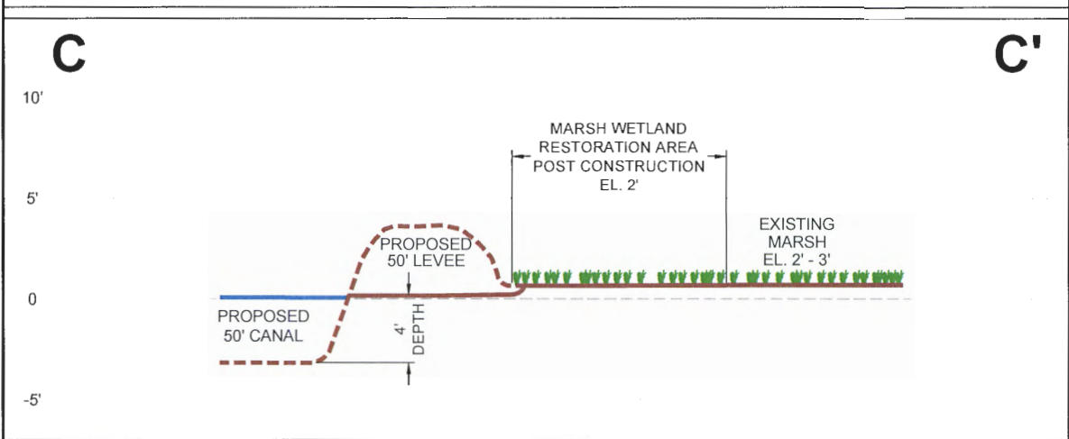
FIGURE 20 REV CROSS SECTIONS A-A' & B-B' OUTFALL AND POST CONSTRUCTION CROSS SECTION C-C' OUTFALL CANAL 1 - WHITE RANCH RECONSTRUCTION OF OUTFALL CANALS CHAMBERS AND JEFFERSON COUNTIES, TEXAS
