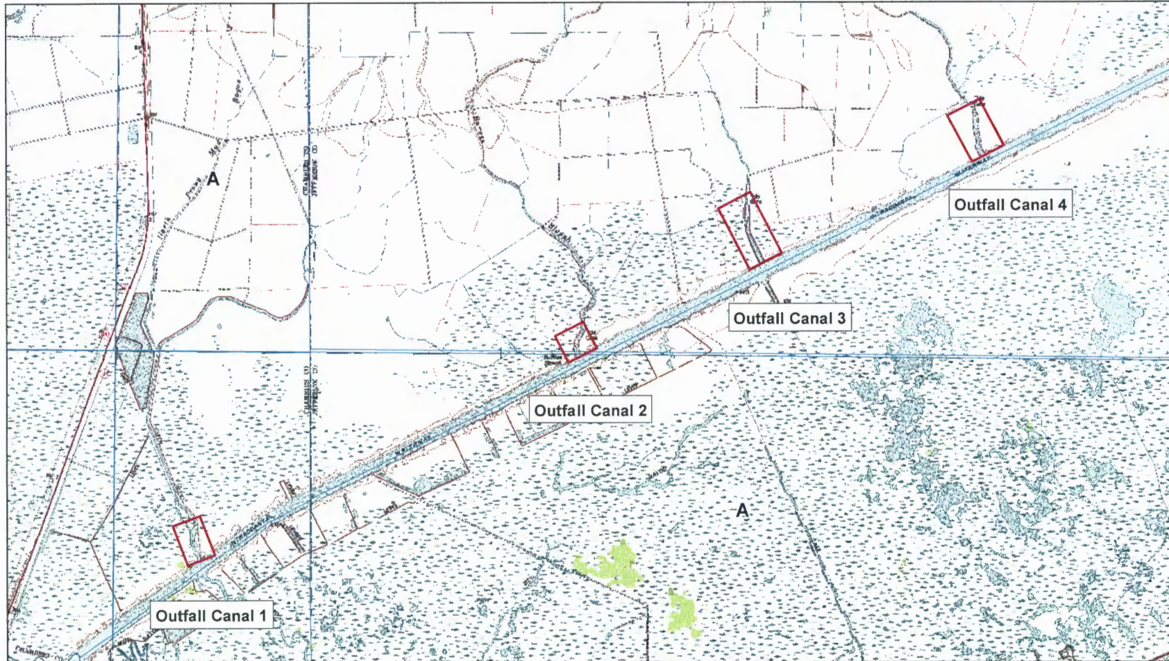
TOPOGRAPHY AND FLOOD MAP RECONSTRUCTION OF OUTFALL CANALS CHAMBERS AND JEFFERSON COUNTIES, TEXAS SWG-2008-00352
