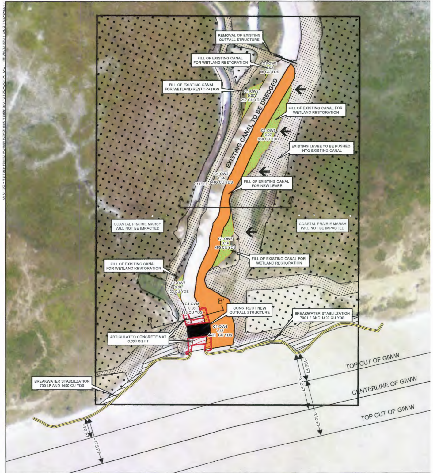
FIGURE 6 REV OUTFALL CANAL 1 RECONSTRUCTION OF OUTFALL CANAL MAP CHAMBERS AND JEFFERSON COUNTIES, TEXAS SWG-2008-00352
