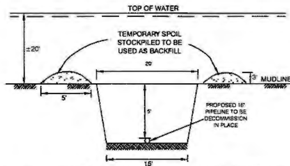
CROSS SECTION VIEW OF TYPICAL TEMPORARY WORKSPACE NOT TO SCALE
