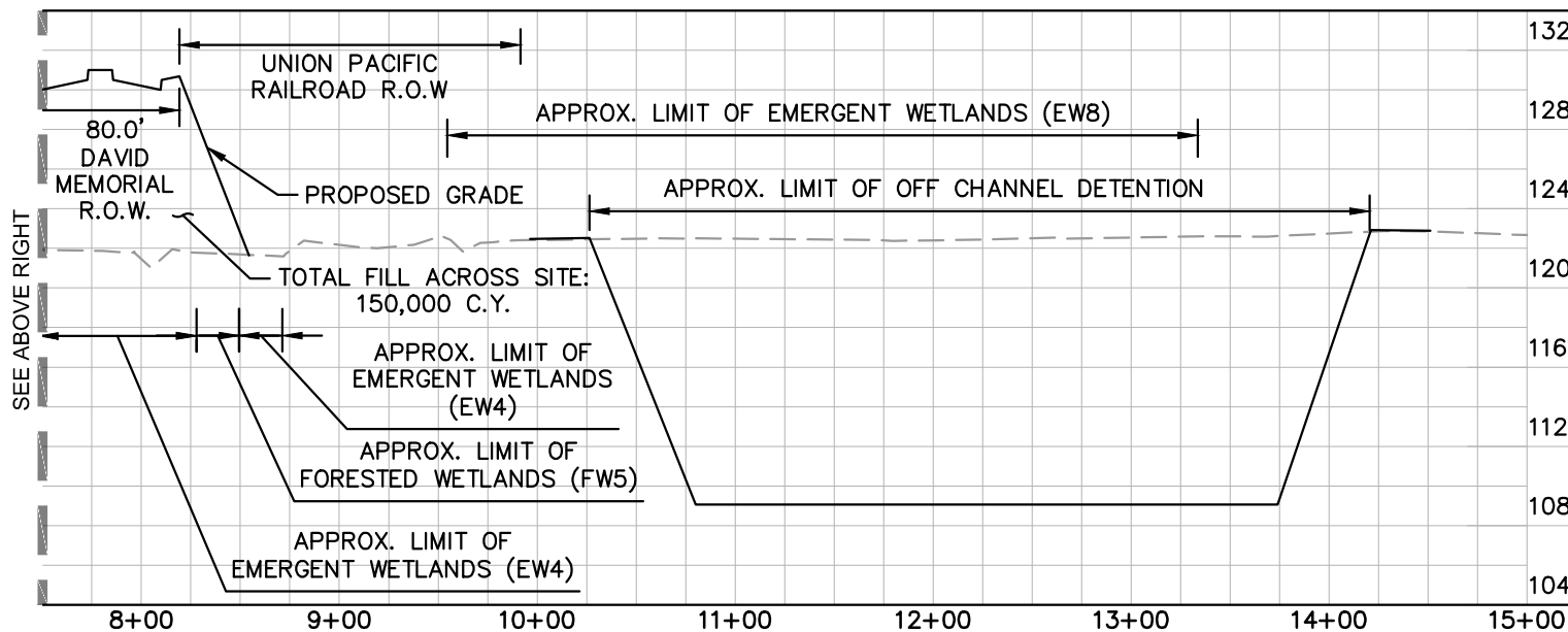
SECTION D-D SCALE 1"=100' H; 1"=10' V
