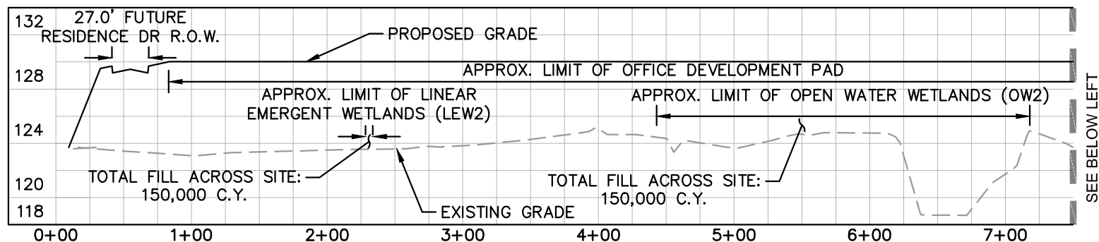
SECTION C-C SCALE 1"=100' H; 1"=10' V
