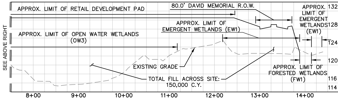
SECTION B-B SCALE 1"=100' H; 1"=10' V
