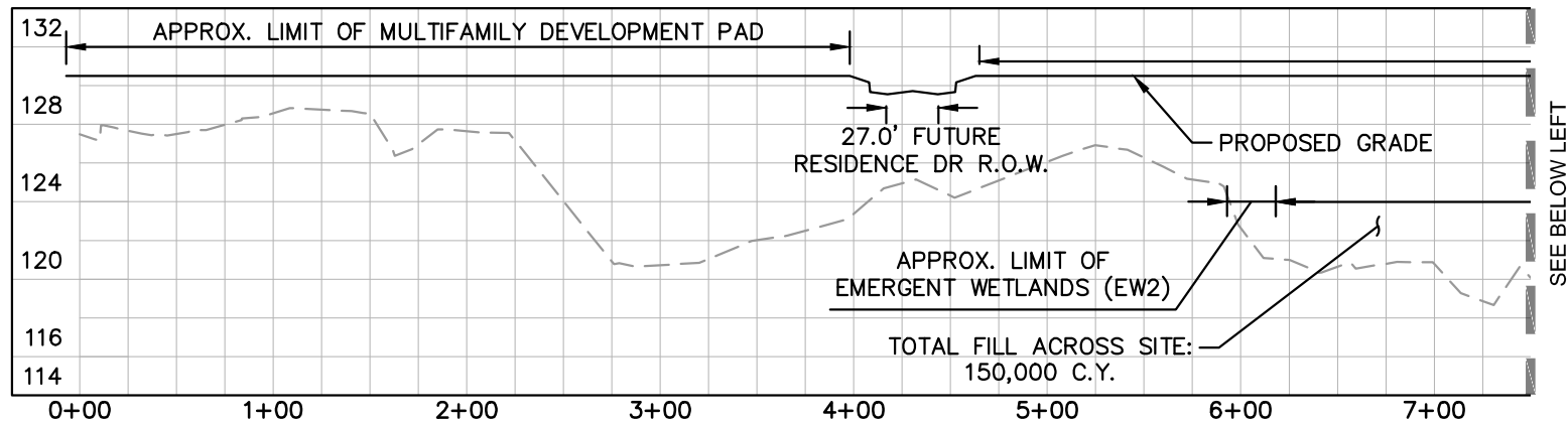
SECTION B-B SCALE 1"=100' H; 1"=10' V
