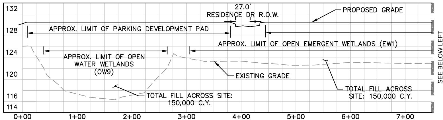
SECTION A-A SCALE 1"=100' H; 1"=10' V
