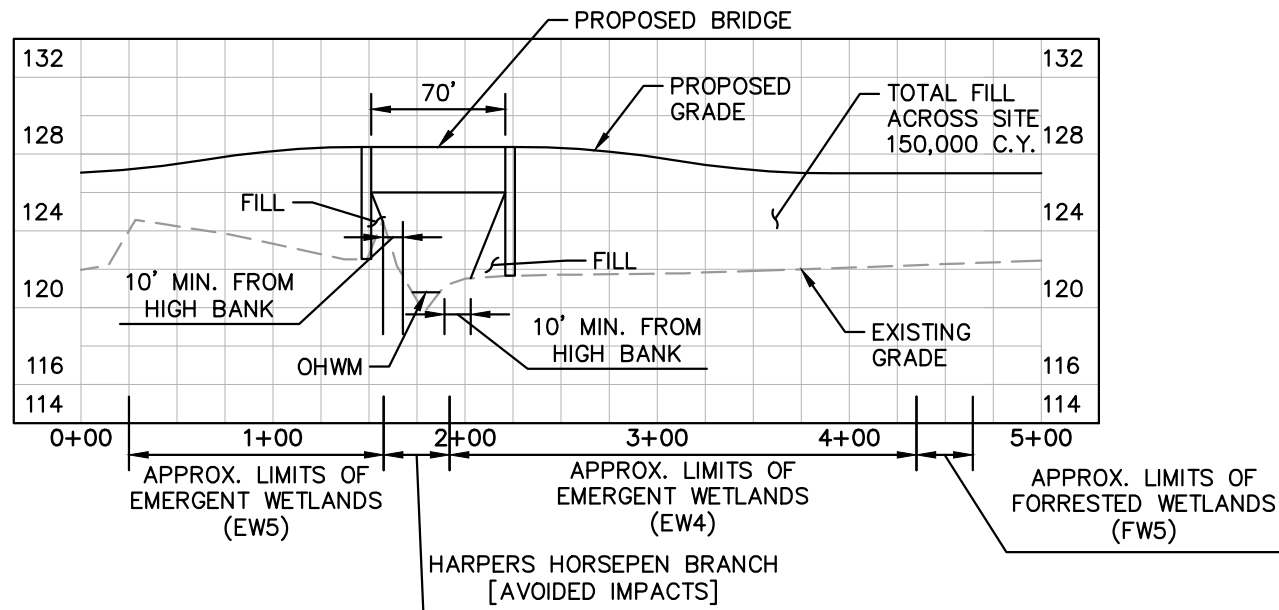
SECTION F-F SCALE 1"=100' H; 1"=10' V
