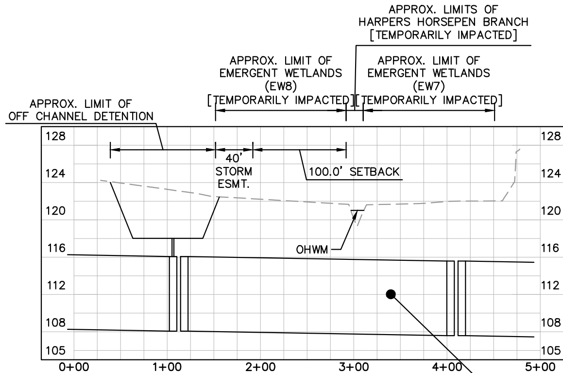
SECTION E-E SCALE 1"=100' H; 1"=10' V
