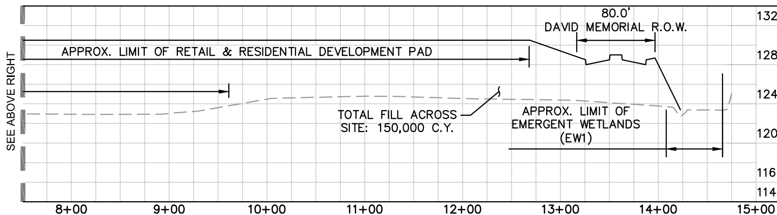
SECTION A-A SCALE 1"=100' H; 1"=10' V
