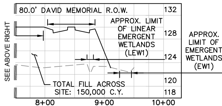
SECTION C-C SCALE 1"=100' H; 1"=10' V
