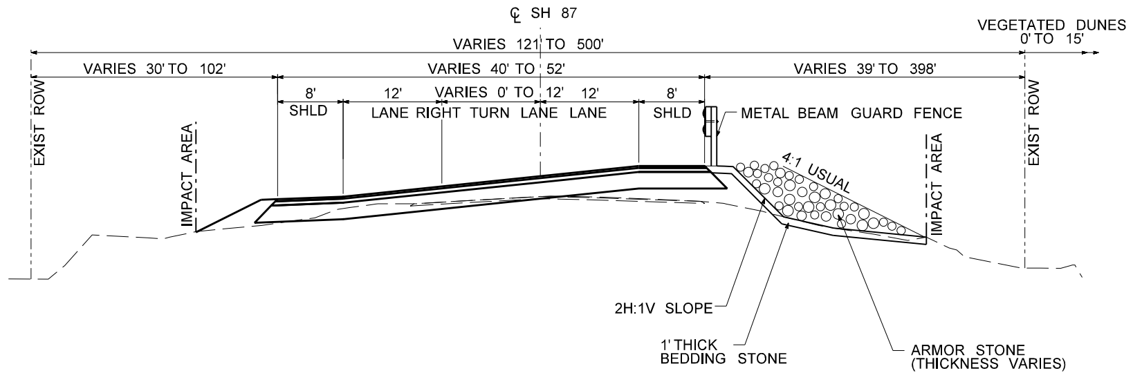
TYPICAL CROSS SECTION WITH ARMORING
