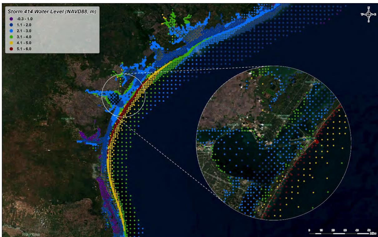
Figure 5: Water levels generated by Storm 414
