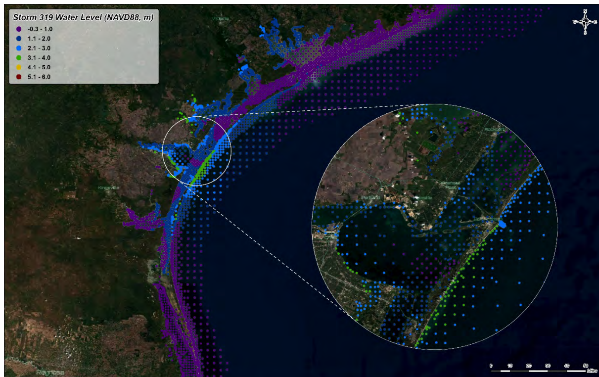
Figure 3: Water levels generated by Storm 319
