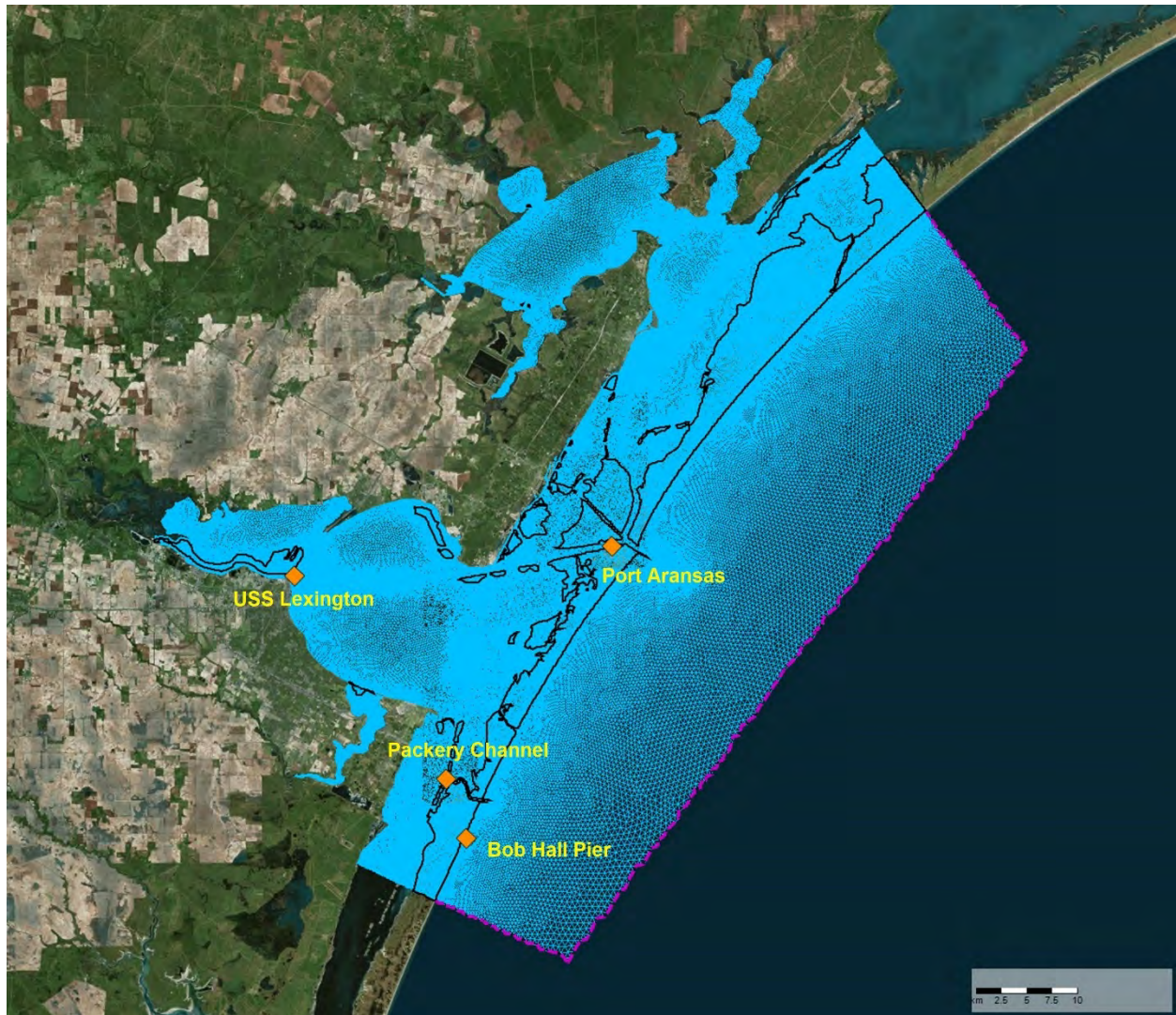
Figure 18. Delft3D-FM model grid is shown in blue. The magenta color shows the offshore boundaries and the black colored polygons show the land boundaries. The orange diamonds show NOAA tide stations used for input to the model (Bob Hall Pier) and water level output validation (Packery Channel, Port Aransas, and USS Lexington).
