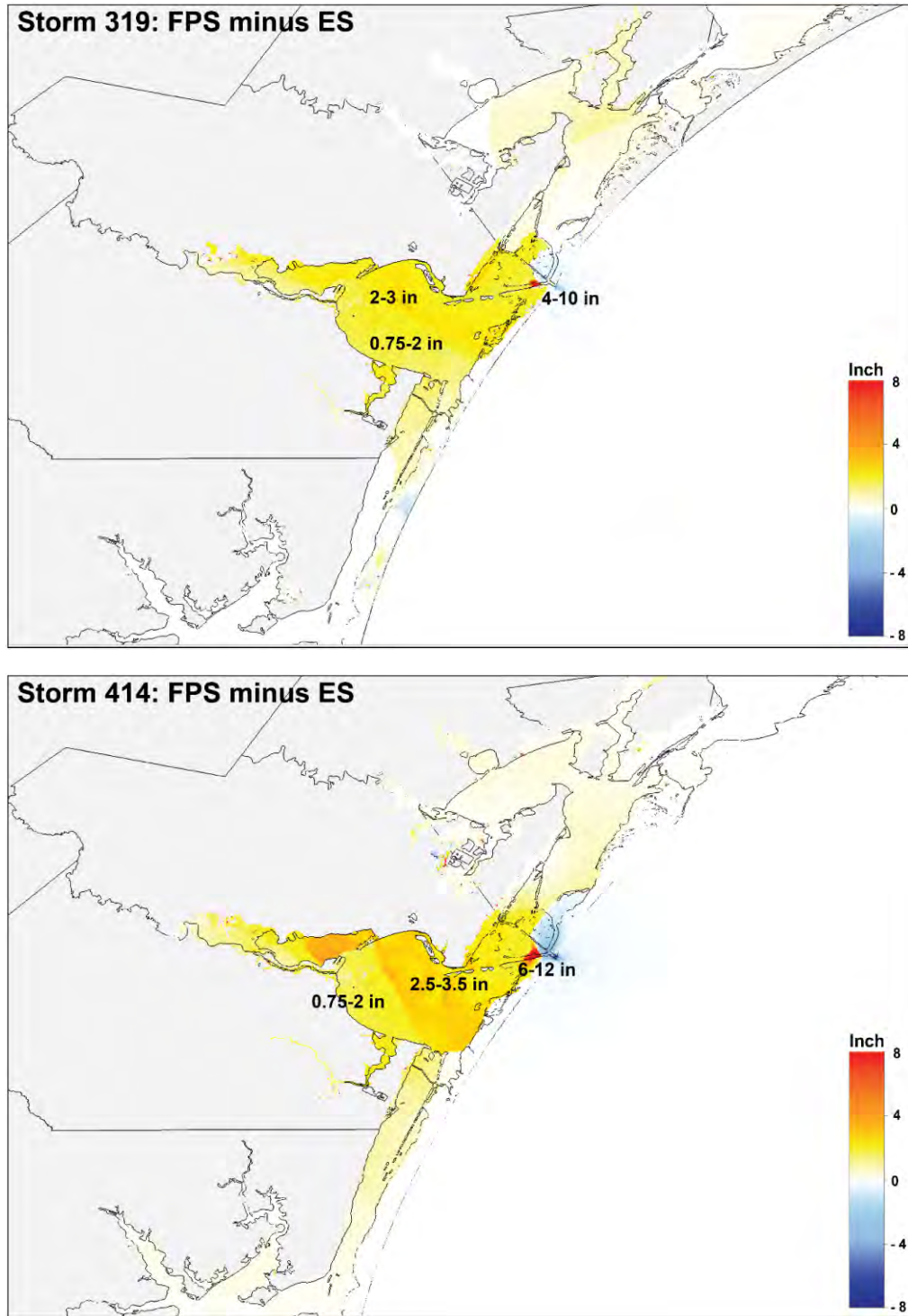
Figure 7: Difference in maxele of Storm 319 FPS and ES (top) and Storm 414 FPS and ES (bottom). Warmer colors indicate higher water level due to the increase in the channel depth in the FPS channel configuration. (Figures taken from HRI “Impacts of Channel Dredging on Storm Surge, Tidal Flows and Salinity in Corpus Christi Bay” report dated April 1, 2021)
