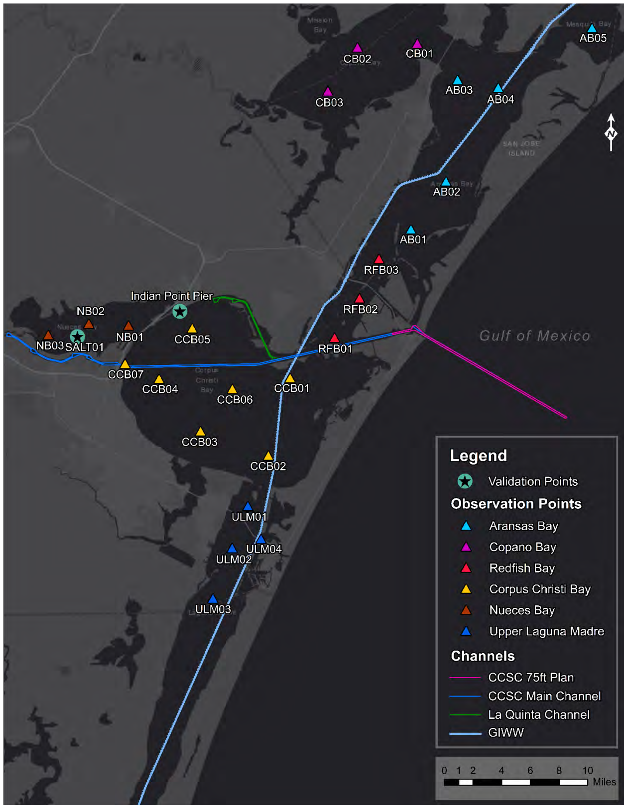
Figure 35. Validation points (Indian Point Pier and SALT01 in Nueces Bay) used for the surface salinity validation and model observation points used for three channel configurations comparison.
