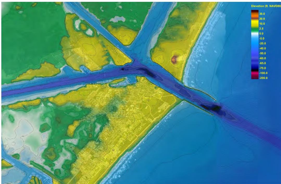
Figure 8: Existing Scenario (ES) bathymetry
