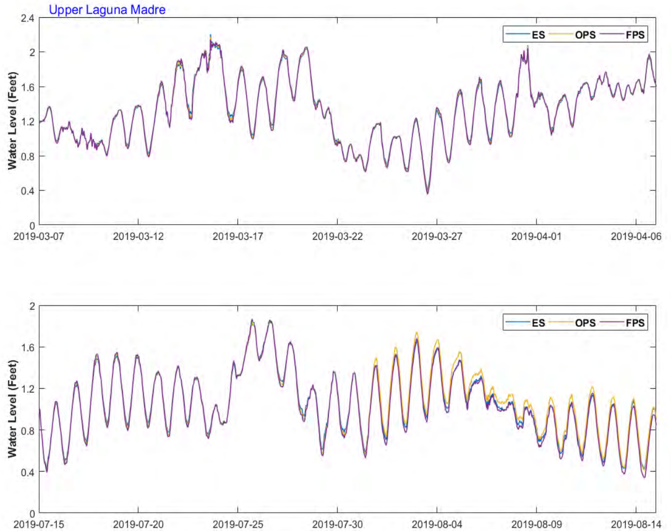
Figure 31. Tide comparison between ES, OPS and FPS at an observation point in the middle of Upper Laguna Madre shown with white box in Figure 27. The top graph is over a 1-month period in Mar/Apr 2019 and the bottom graph is over a 1-month period in Jul/Aug 2019.
