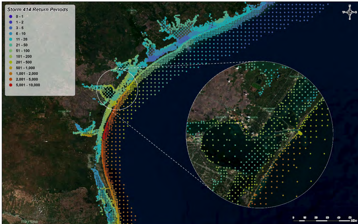
Figure 6: Return periods associated with the Storm 414 water levels (non-exceedance limit: %90)
