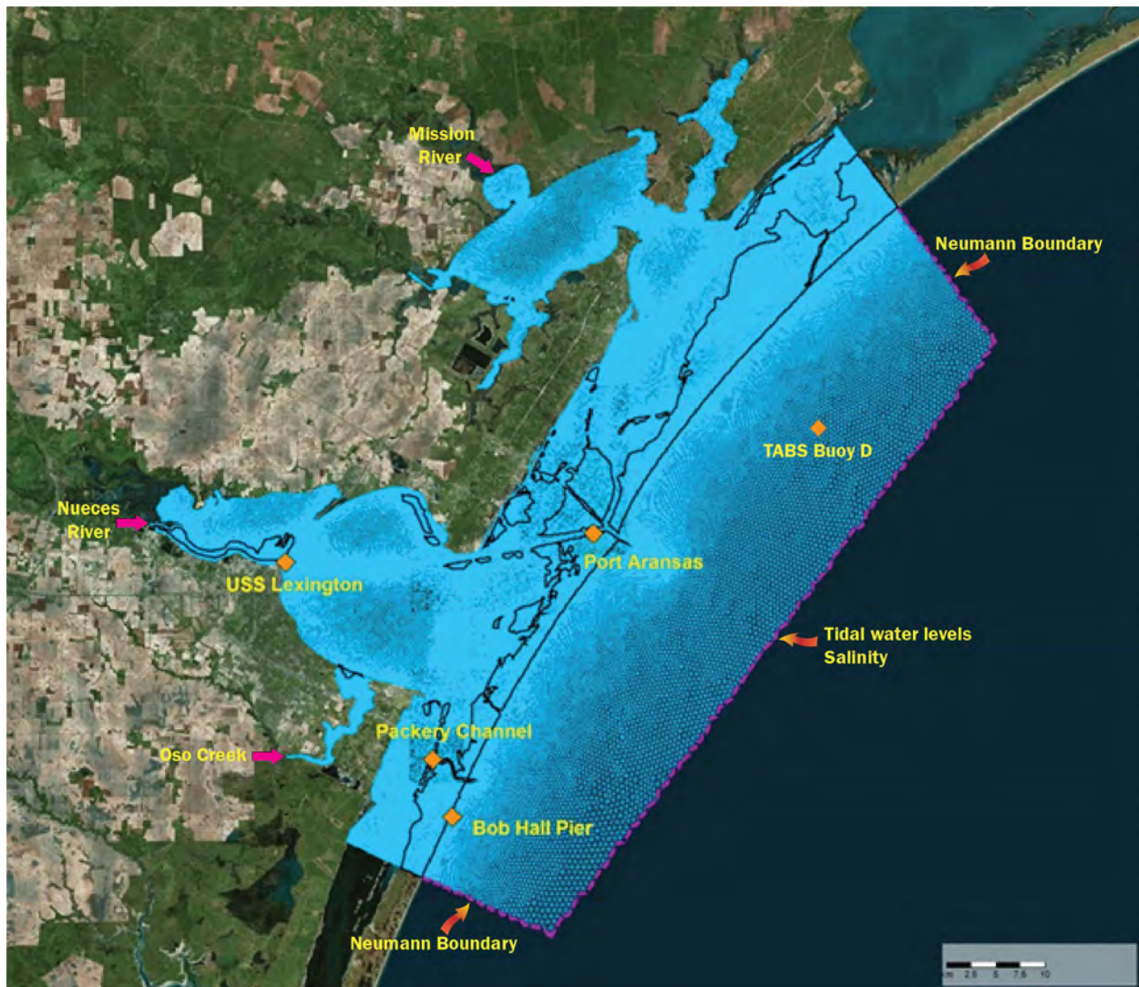
Figure 34. Delft3D-FM model grid is shown in blue. The magenta color shows the offshore boundaries, and the black colored polygons show the land boundaries. The model is driven with tidal water levels from Bob Hall Pier, surface salinity from Buoy D, and river flows from Oso Creek, Nueces River and Mission River (shown with pink arrows).
