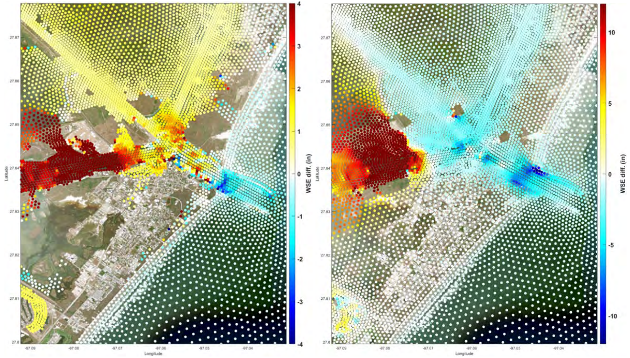
Figure 12: Storm 319 (left) and Storm 414 (right) water surface elevation (WSE) difference between FPS and ES (FPS minus ES) at model output timestep 130/168 and 84/96 respectively. Units in inches.
