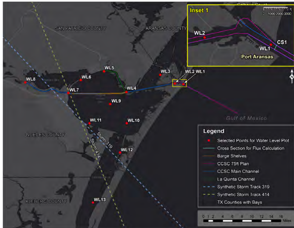
Figure 1: Study area map showing hurricane tracks (Figure taken from HRI “Impacts of Channel Dredging on Storm Surge, Tidal Flows and Salinity in Corpus Christi Bay” report dated April 1, 2021)
